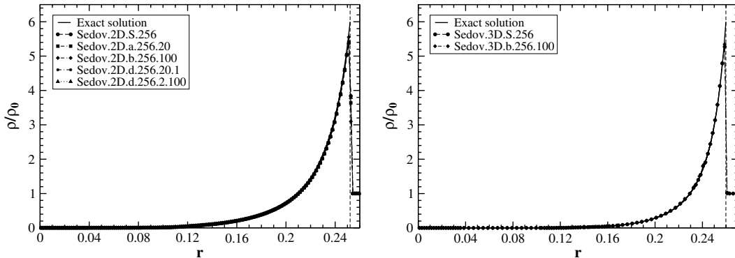
Fig. 2. Left: Comparison of runs Sedov.2D at time t_{tot} = 0.9975 \times 10^{-3} . Right: Comparison of runs Sedov.3D at time t_{tot} = 0.355 \times 10^{-3} . In both panels shown is density along the diagonal cut of the computational domain in the units of ambient density \rho_0 . Vertical dashed line indicates the shock front position based on the exact solution.
