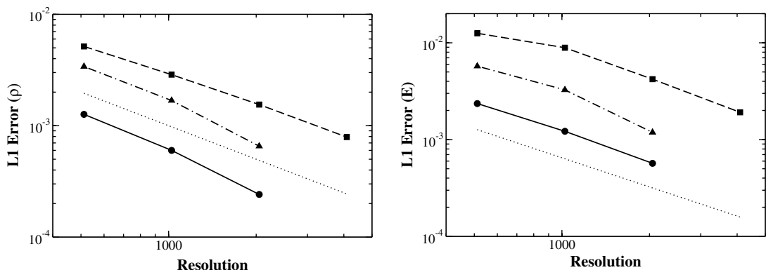
Fig. 11. Convergence of the L1 error in density (left) and total energy (right) for the simulations of expansion of a rotating sphere into vacuum. Dotted lines show the expected rate of convergence. Left: Circles: convergence of runs SphereRot.2D.S.512–2048.80 to the run SphereRot.2D.S.4096 at t = 0.02 (order of convergence O(1.13) ); Squares: convergence of runs SphereRot.2D.e 2 .256–2048.80 to the run SphereRot.2D.S.4096 at t = 0.02 ( O(0.87) ); Triangles: convergence of runs SphereRot.2D.e 2 .256–1024.80 to the run SphereRot.2D.e 2 .2048.80 at t = 0.75 ( O(1.1) ). Right: Order of convergence: Circles – O(0.99) ; Squares – O(0.76) ; Triangles – O(0.98) .
