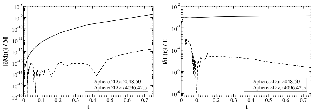
Fig. 8. Temporal evolution of the relative error in total mass (left) and total energy (right) conservation for the simulations of expansion of a non-rotating sphere into vacuum. Vertical line indicates the time of start of the reference frame expansion for the run Sphere.2D.a j .4096.42.5.
