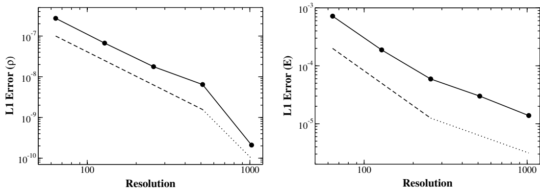
Fig. 12. Convergence of the L_1 error in density (left) and total energy (right) in runs Clump.2D.a.*.100. Dashed line in both panels corresponds to second-order convergence, while the dotted line in the left panel corresponds to fourth-order convergence and in the right panel – to first-order convergence. Overall convergence order in density is O(2.01) and total energy is O(1.88) .
