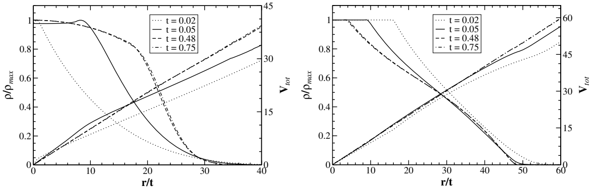
Fig. 5. Left: Run Sphere.2D.a.2048.50. Right: Run SphereRot.2D.e2.2048.80. Both panels show normalized density (set of decreasing curves) and total velocity (set of increasing curves). Density is normalized to its maximum value at each time. All distributions are given along the diagonal cut of the domain.
