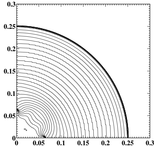
Fig. 1. Contour plot of the density logarithm for the run Sedov.2D.b.256.100 at time t_{tot} = 0.9975 \times 10^{-3} (cf. Fig. 2). 30 contour lines correspond to the values of the density logarithm that are equally spaced between its maximum (0.75) and minimum (-3.11) values.
