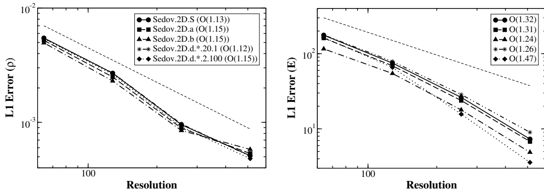
Fig. 7. Convergence of the numerical solution to the exact one in simulations of the Sedov blast wave in various reference frames. Left: L_1 error in density. Right: L_1 error in total energy in the laboratory reference frame. The order of convergence is shown in brackets in the legend in both panels. The dashed lines correspond to first-order convergence.
