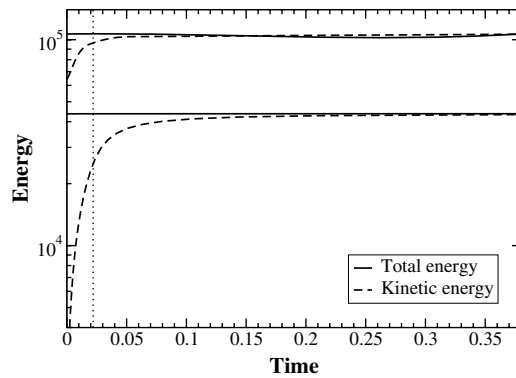
Fig. 6. Temporal evolution of the kinetic energy in the case of expansion of a non-rotating sphere (lower pair of curves, run Sphere.2D.a.2048.50) and a rotating sphere (upper pair of curves, run SphereRot.2D.e2.2048.80) into vacuum. Shown only the first half of the total physical simulation run time. Vertical dashed line corresponds to the total run time of the runs Sphere.2D.S and SphereRot.2D.S.
