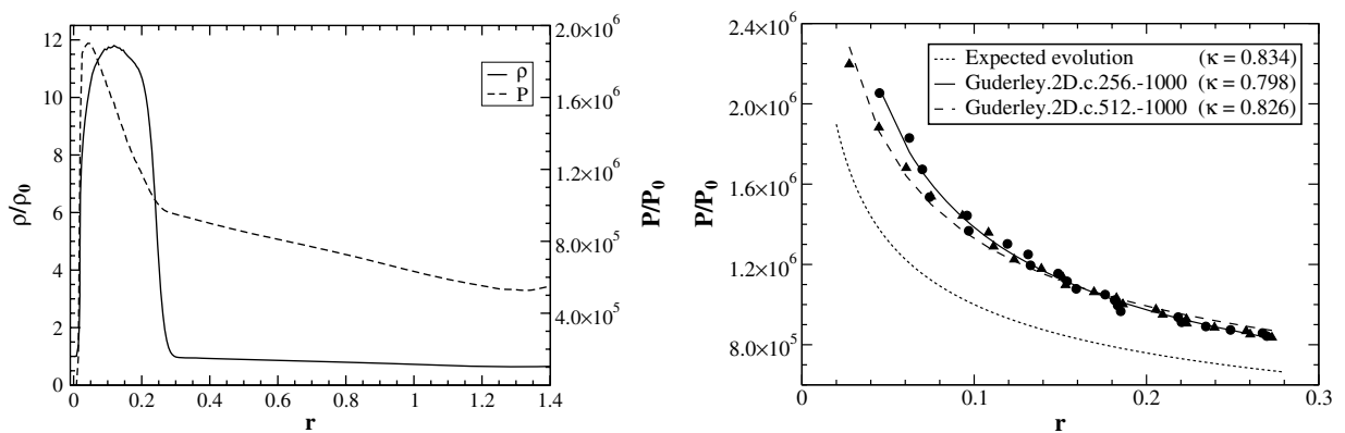
Fig. 3. Left: Structure of the converging shock wave right before the shock front collapse at the center of symmetry. Shown is density and pressure, normalized to their pre-shock values \rho_0 and P_0 , at time t = 0.89 \times 10^{-3} . Profiles are taken along the diagonal cut of the computational domain of the run Guderley.2D.S.256. Right: Position and values of pressure maxima for the final stages of collapse of the converging shock. Circles represent pressure maxima at each moment in time for the run Guderley.2D.c.256.–1000, while the triangles show the same for the run Guderley.2D.c.512.–1000. The solid and dashed lines show the corresponding fits for those two runs. The dotted line shows the expected evolution.
