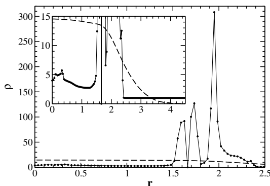
Fig. 13. Test Sphere.2D.a.256.50 performed with Zeus-MP (solid line). Shown is the diagonal cut through the domain at t = 0.12 . Dashed line shows the reference solution obtained with the method presented here. Inset shows the zoom-in of the main graph.
