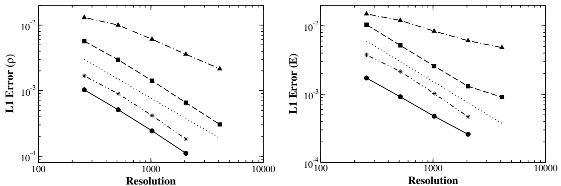
Fig. 10. Convergence of the L1 error in density (left) and total energy (right) for the simulations of expansion of a non-rotating sphere into vacuum. Dotted lines show the expected rate of convergence. Left: Circles: convergence of runs Sphere.2D.S.256–2048 to the run Sphere.2D.S.4096 at t = 0.024 (order of convergence O(1.04) ); Squares: convergence of runs Sphere.2D.a.128–2048.50 to the run Sphere.2D.S.4096 at t = 0.024 ( O(1.0) ); Triangles: convergence of runs Sphere.2D.a.128–2048.50 to the run Sphere.2D.a.d.4096.42.5 at t = 0.75 ( O(0.6) ); Stars: convergence of runs Sphere.2D.a.d.256–2048.42.5 to the run Sphere.2D.a.d.4096.42.5 at t = 0.75 ( O(0.98) ). Right: Order of convergence: Circles – O(0.92) ; Squares – O(0.99) ; Triangles – O(0.42) ; Stars – O(0.92) .
